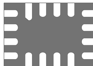
QFN1826-16L
