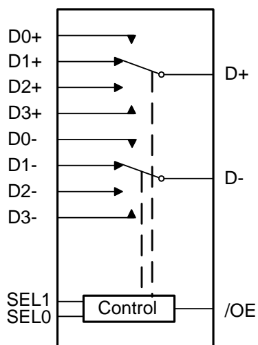
Logic Symbol
